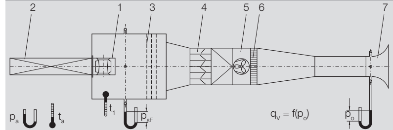
Fan curves measurement RZR - ISO 5801 / DIN 24163
