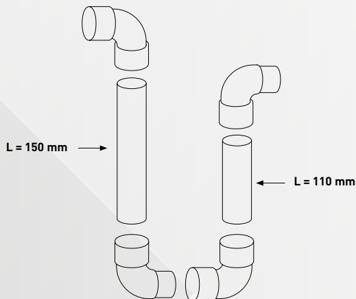
Figure 16a Raccordement du siphon de surpression
