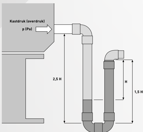
Figure 16b Raccordement du siphon de surpression
