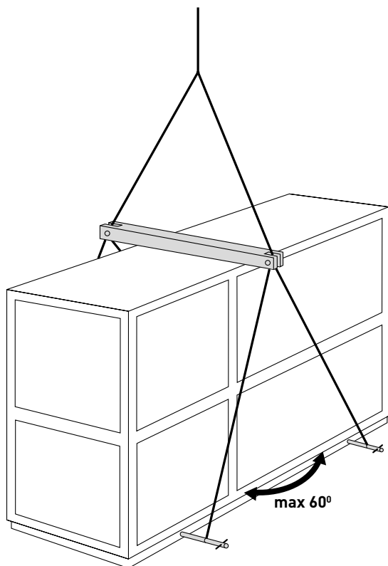
Figure 2 Instructions de levage
